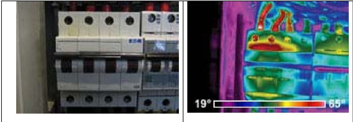
Inspection of this fuse box discovers that the two left connections are overheated.
