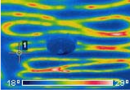
Hot spots in the ceiling
