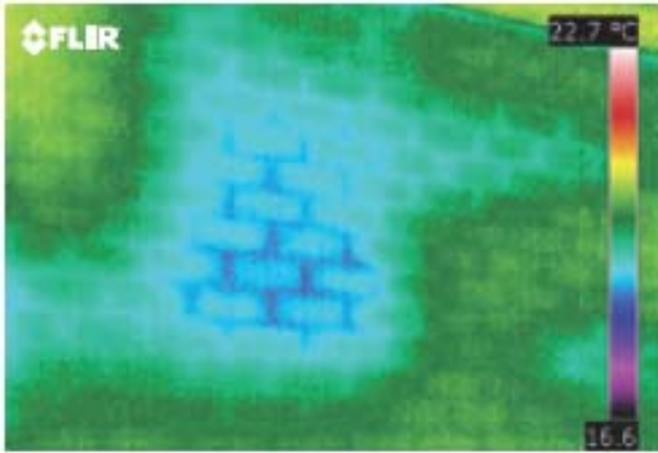
Missing insulation in parts of the wall.
