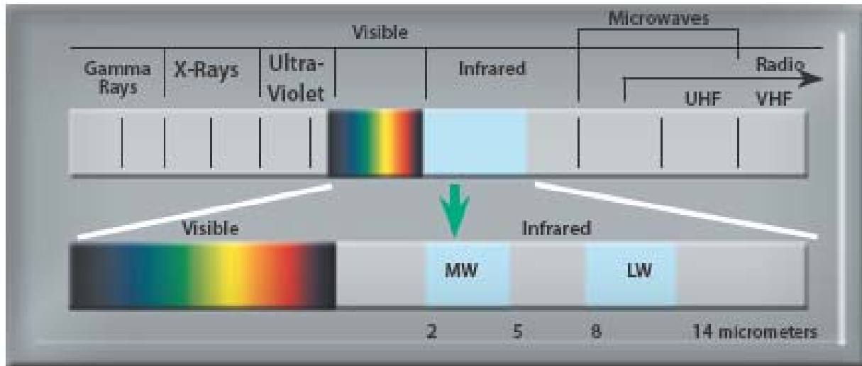
Electromagnetic Spectrum
